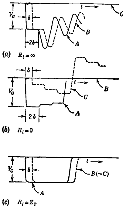
FIG. 12-18.—Drawings of synchroscope traces obtained at points A, B, and C in the circuit of Fig. 12-17 for three different values of R_1 .
